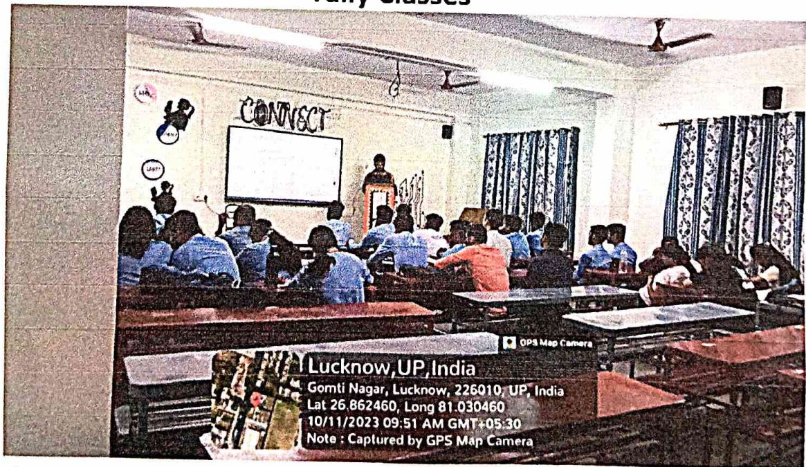
Python Classes
