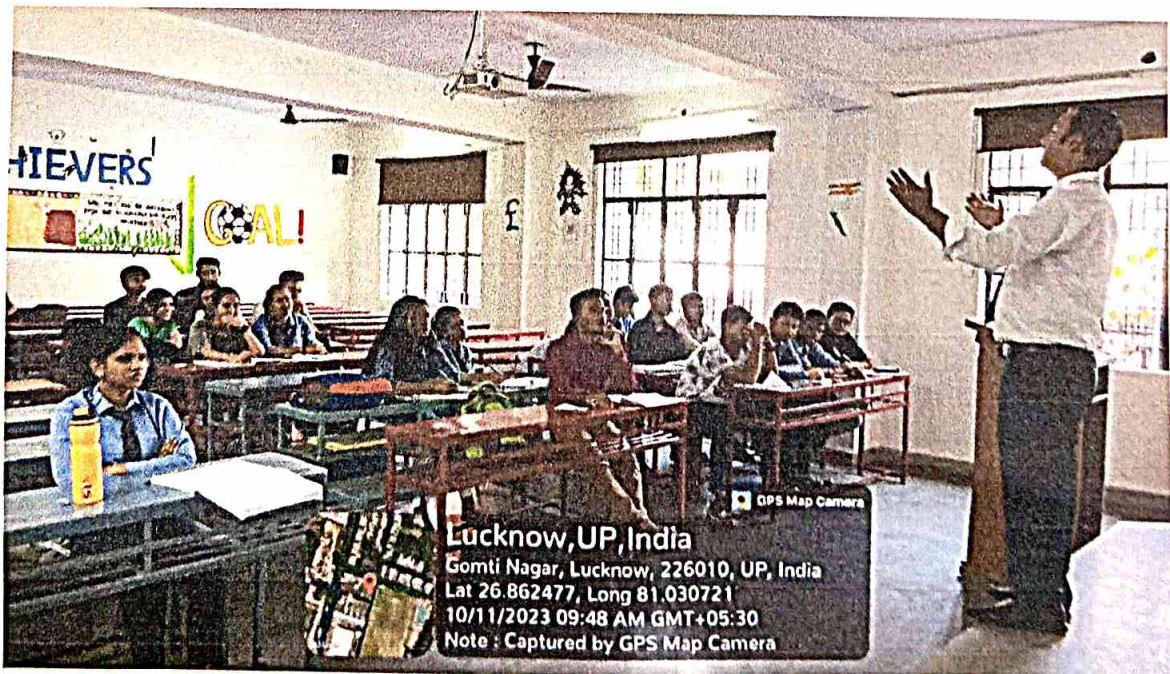
French Classes
