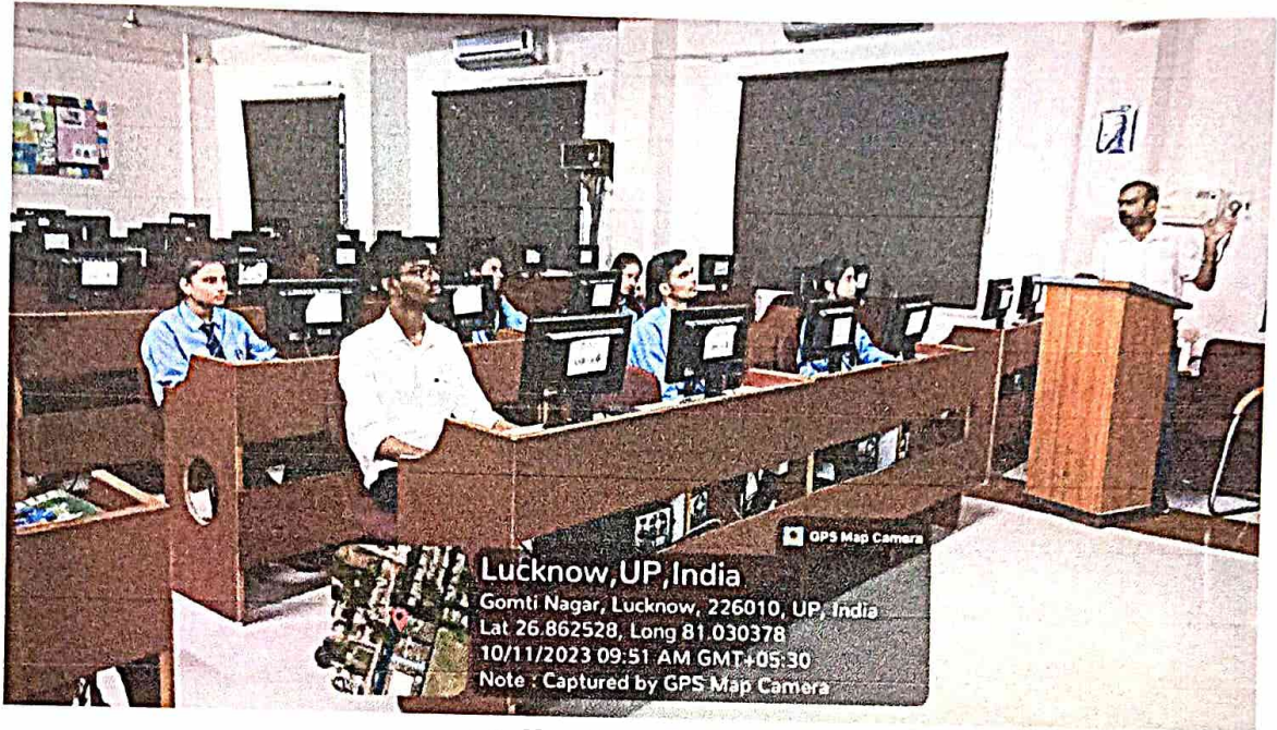
Tally Classes
